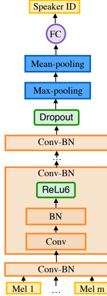
Figure 10: Architecture for speaker discriminator.
