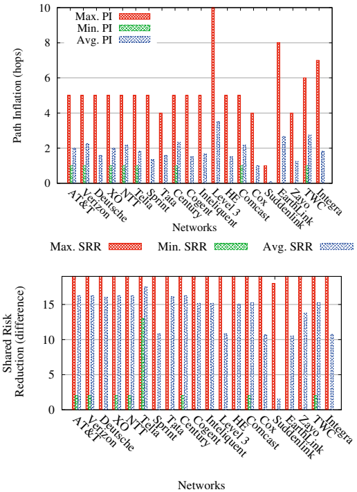
Figure 10: Path Inflation (top) and Shared Risk Reduction (bottom) based on the robustness suggestion framework for the twelve heavily shared links.
