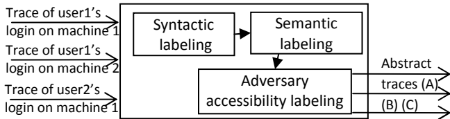
Figure 6: input, output and the three steps of the BRM analyzer
