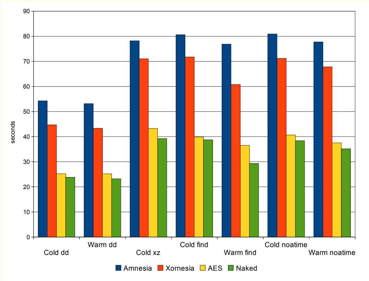
Figure 3: Loop-Amnesia Performance
